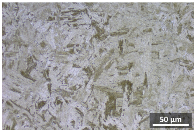
Microstructure after heat treatment at 1090°C/30min/Quench + 680°C/4h/Air giving a hardness of 48 HRC.
