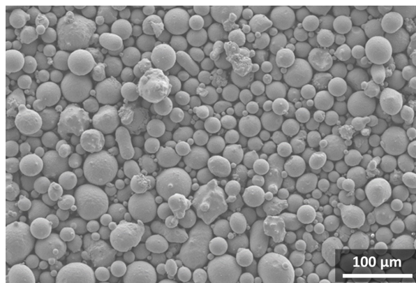
Typical powder morphology.
