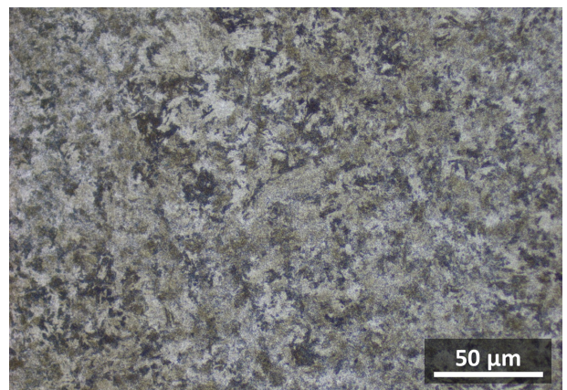
Microstructure after heat treatment at 845°C/30min/Air + 610°C/4h giving a hardness of 44.5 HRC
