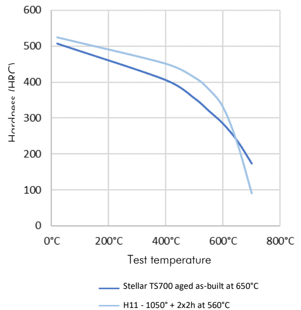
HARDNESS AT TEMPERATURE
