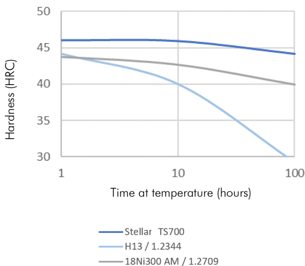
THERMAL SOFTENING AT 600°C
