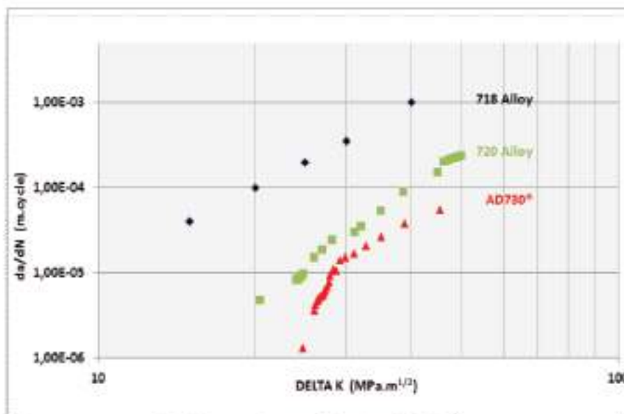
Crack growth rates of various C&W alloys Temperature 650°C (1202°F); Stress Load Ratio R=0.1; Trapezoidal wave form with 300 seconds at the peak load ( 10s-300s-10s)
