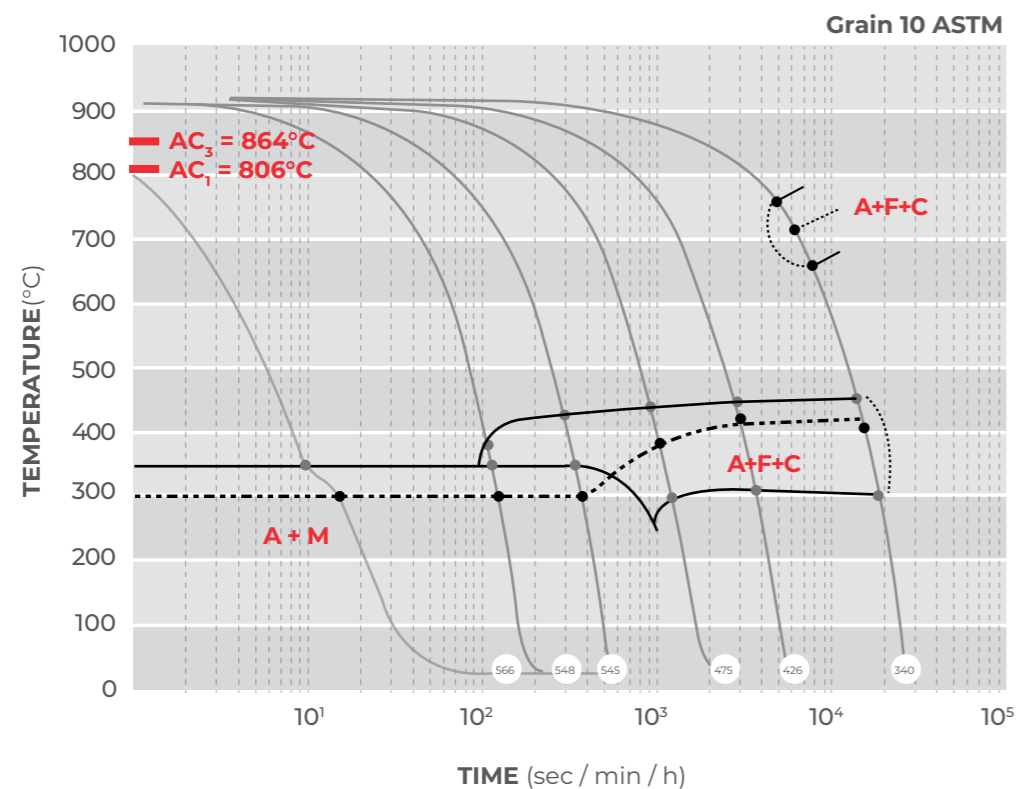
CCT Diagram (austenitization 920°C, 1688°F)
